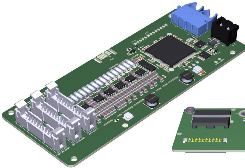
Single channel baseboard for up to 3 modules in
