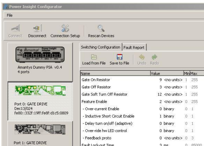
Figure [2] – Example of Configuration Pane in Amantys Power Insight Configurator
